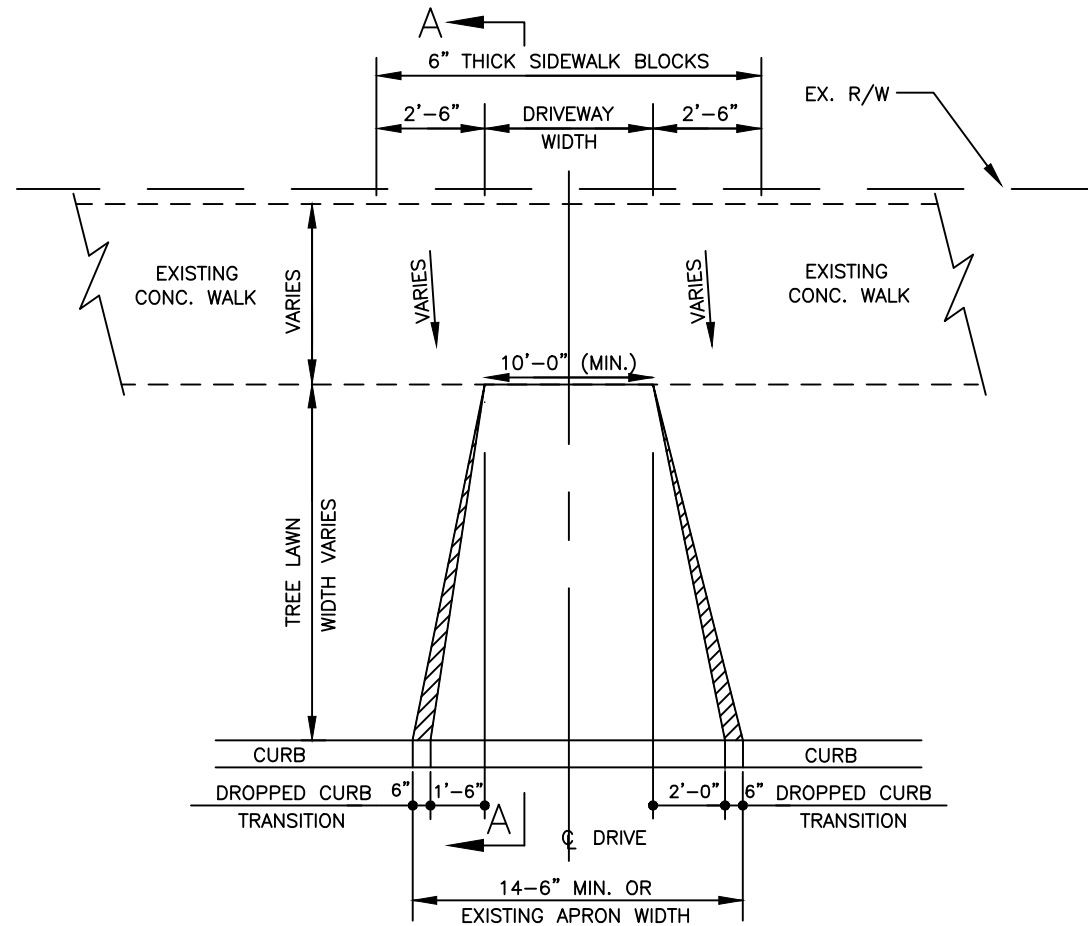
DRIVE APRON DETAIL TREELAWN GREATER THAN 6'-0"
