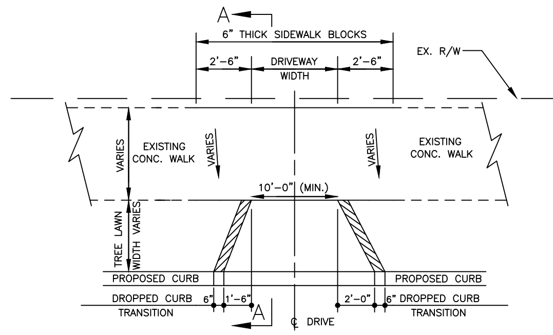
DRIVE APRON DETAIL TREELAWN LESS THAN 6'-0"
