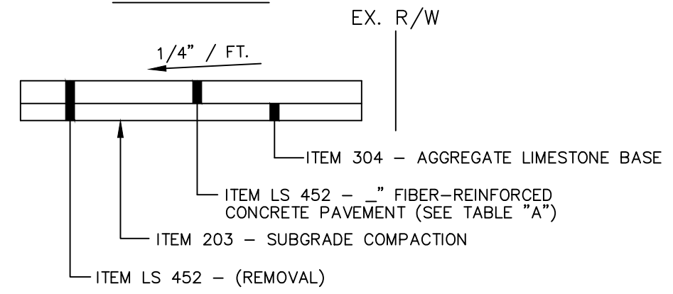
A SECTION
